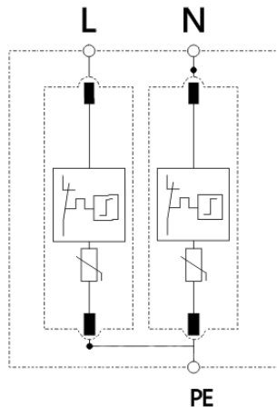
Electrical principle
