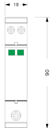
Outline dimension
