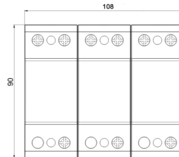
Dimension drawing
