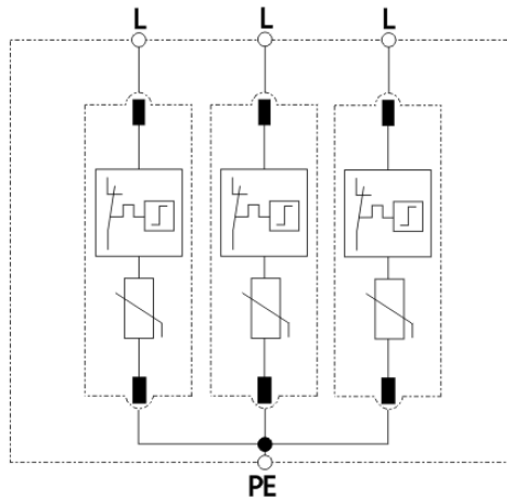
Electrical principle
