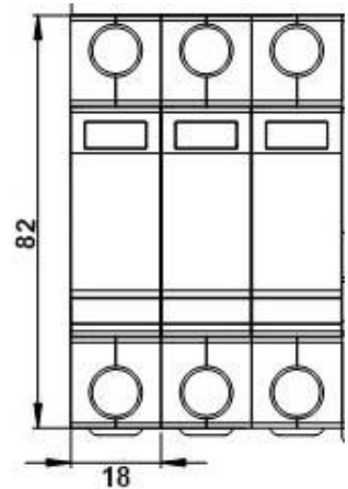
Outline dimension
