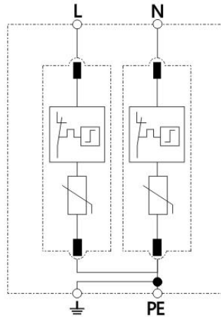
Electrical principle
